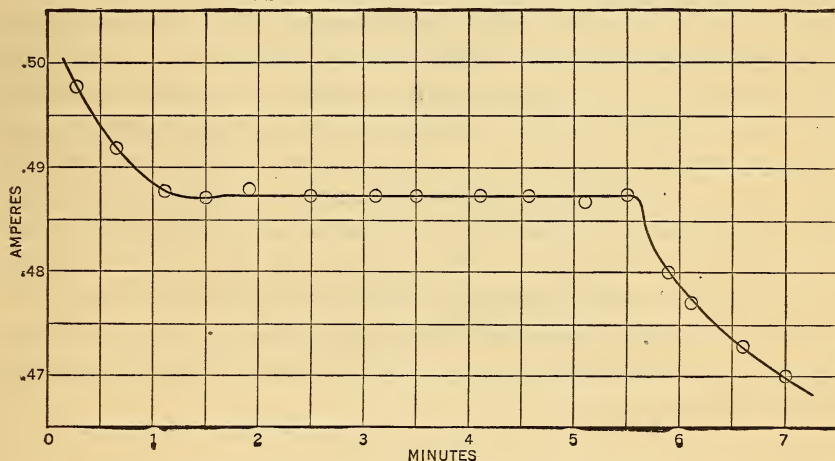
Fig 3.—Calibration of lamp at freezing point of silver
